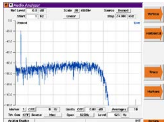
Figure 6. Audio Analyzer
